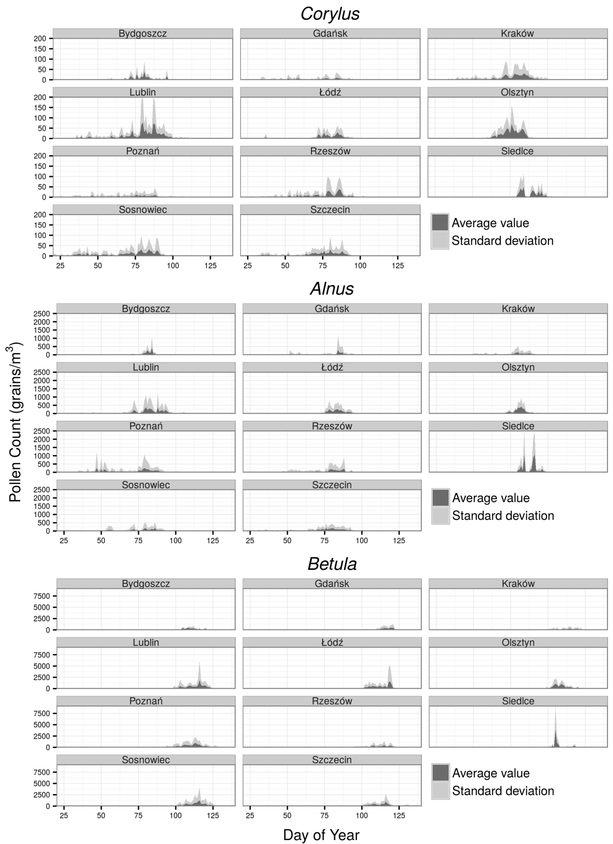
Figure 4: Average value of pollen counts of Corylus , Alnus , and Betula for all of the analyzed years in each location. One standard deviation of pollen count values is represented by the light grey area
