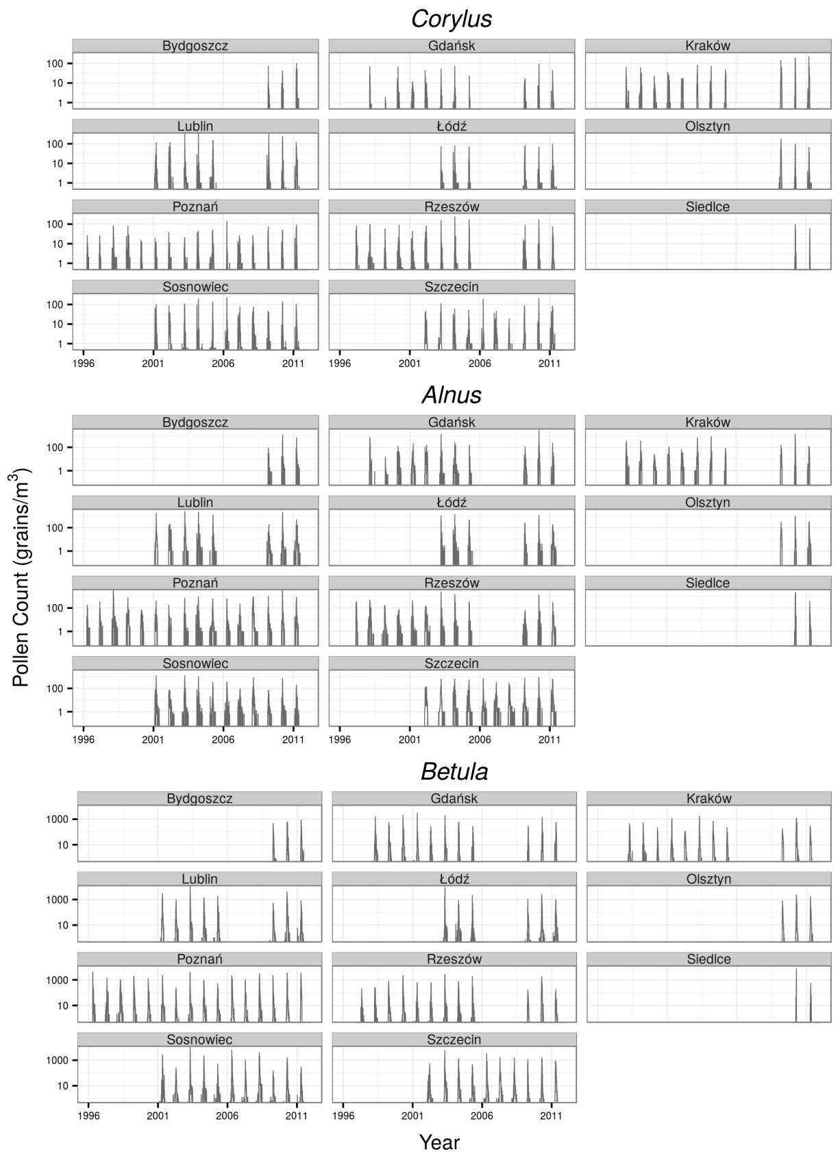
Figure 3: Pollen counts of Corylus , Alnus , and Betula for all of the analyzed years in each location on a logarithmic scale
