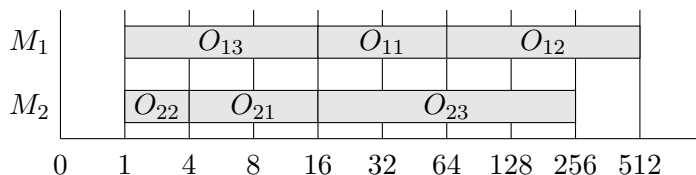
Figure 1. Schedule generated by the LADR rule for instance in Table 1
