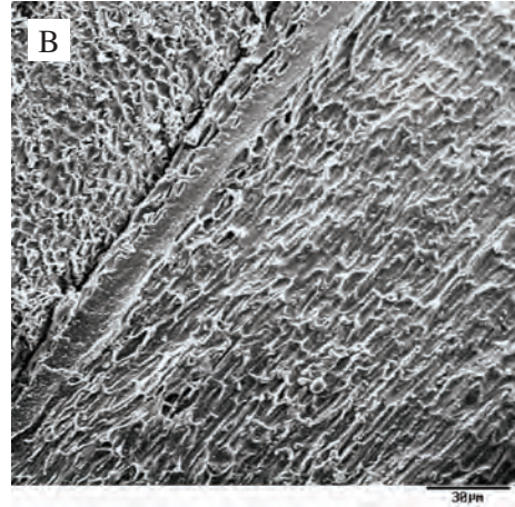
Photo. 1. Scanning electron microscopy (SEM) for contemporary birch bark: (a) x 200, (b) enlargement x 400
