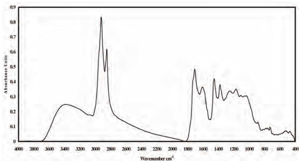
Fig. 14. A typical infrared spectrum of wood-tar substances of technological group I
