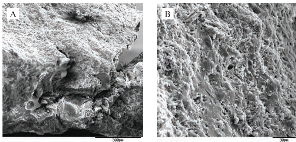
Photo. 53. SEM for sample Sr 39: (a) enlargement x 130, (b) enlargement x 500
