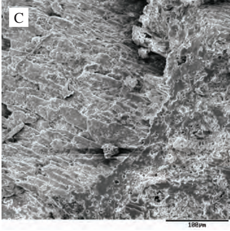
Photo. 16. SEM for sample Sr 327: (c) enlargement x 500
