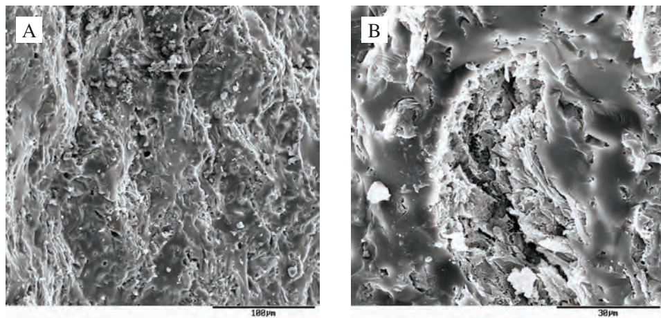
Photo. 52. SEM for sample Sr 184: (a) enlargement x 250, (b) enlargement x 500
