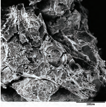
Photo. 12. SEM for sample Sr 92 – enlargement x 250
