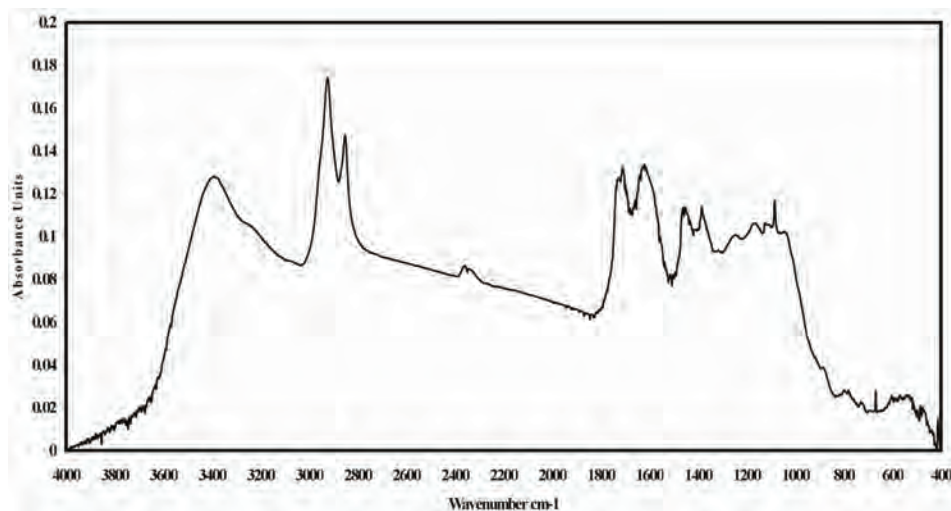
Fig. 15. A typical infrared spectrum (FTIR) of Group II wood-tar substances
