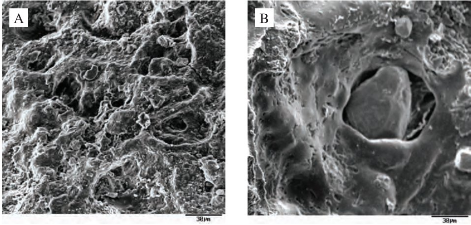
Photo. 45. SEM for sample Sr 454: (a) enlargement x 500, (b) enlargement x 600
