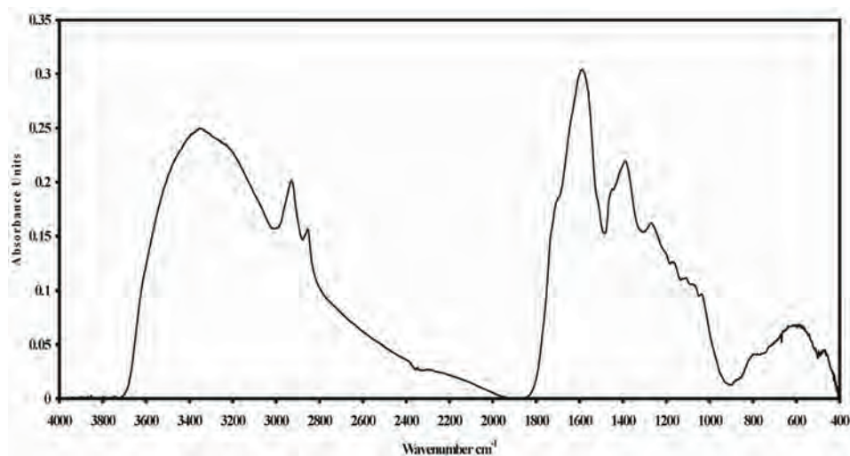
Fig. 16. A typical infrared spectrum of Group III wood-tar substances
