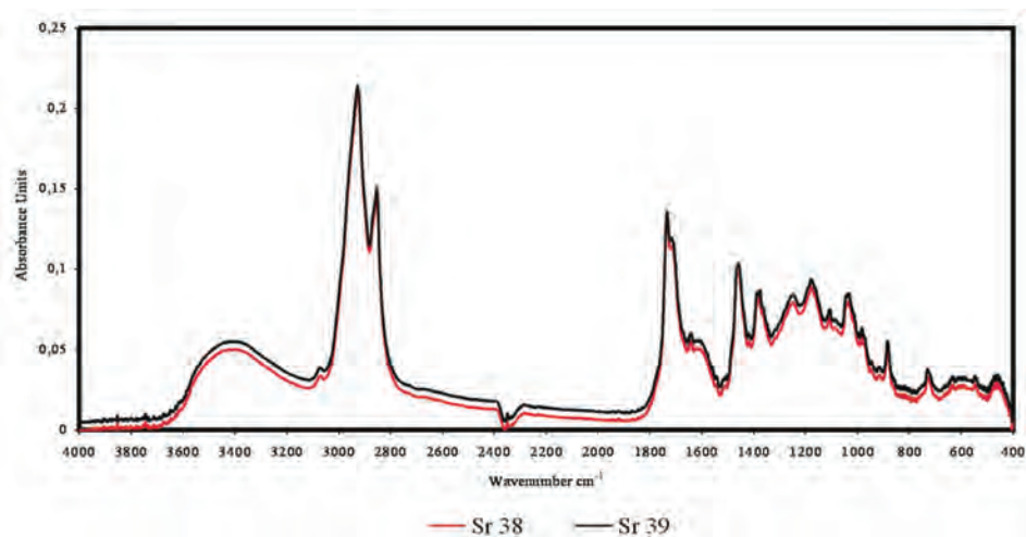
Fig. 21. Infrared spectroscopy correlation for Sr 38 and Sr 39
