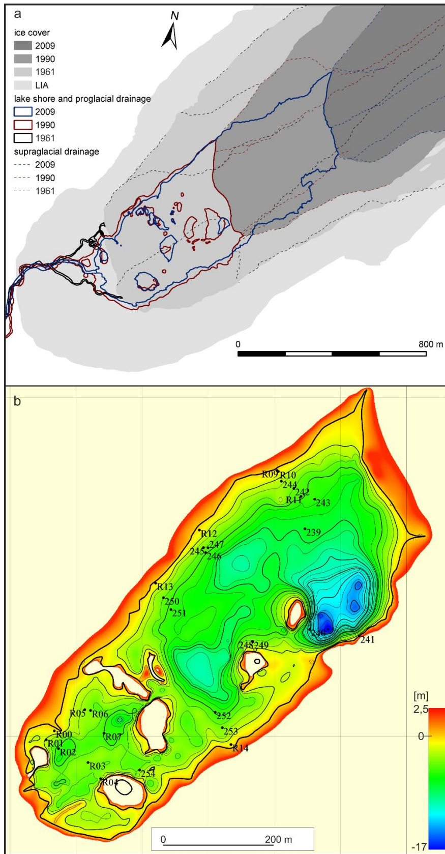
Figure 5. Evolution of the terminoglacial lake, Ragnarbreen, Svalbard; (a) lake shorelines and drainage for different dates; (b) lake bathymetry in 2005 (surveyed by J. Czerniawska, M. Ewertowski, W. Szczuciński)
