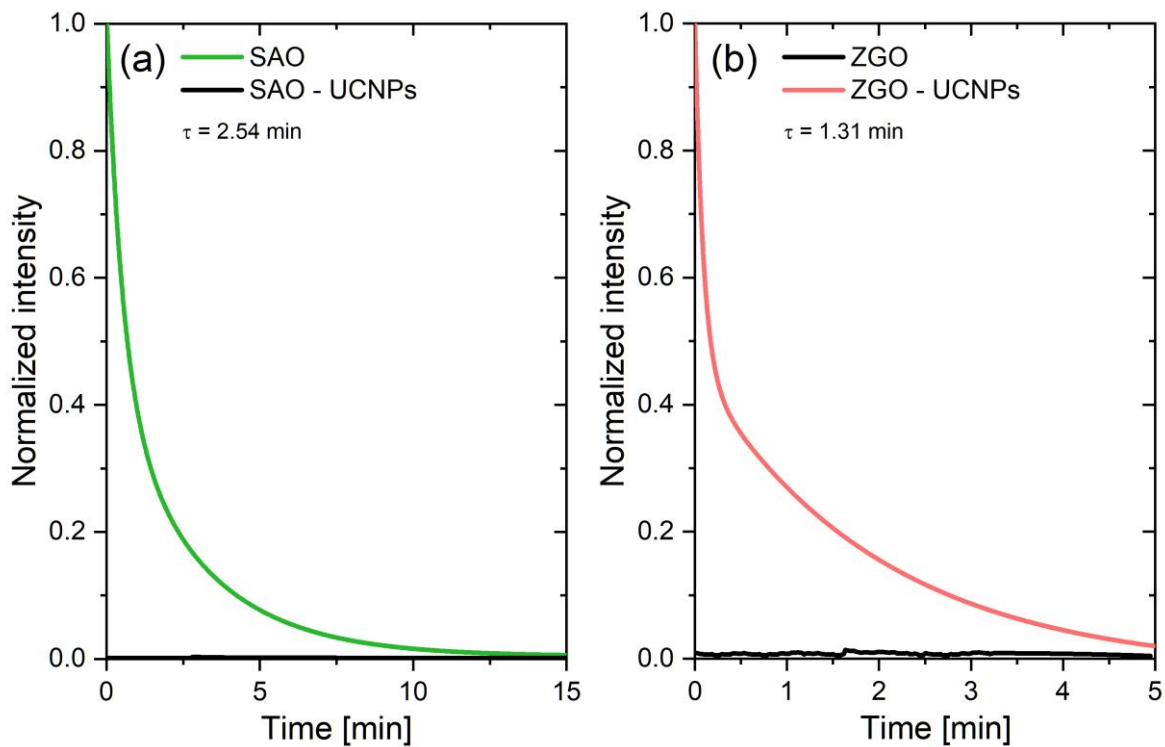
Fig. S1. Normalized decay curves of (a) \text{SrAl}_2\text{O}_4:\text{Eu}^{2+},\text{Dy}^{3+} (SAO), \text{SrAl}_2\text{O}_4:1\%\text{Eu}^{2+},0.5\%\text{Dy}^{3+} -UCNPs (SAO-UCNPs) and (b) \text{ZnGa}_2\text{O}_4:0.5\%\text{Cr}^{3+} (ZGO) and the composite \text{ZnGa}_2\text{O}_4:0.5\%\text{Cr}^{3+} -UCNPs (ZGO-UCNPs) materials after 5 min irradiation with a 975 nm laser with a power density of 6 \text{ W}\cdot\text{cm}^{-2} . The curves for ZGO and SAO were normalized by dividing them by the maximum emission intensity of the corresponding sample containing UCNPs.
