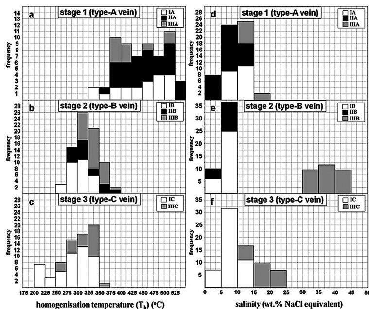
Fig. 5. Histograms of homogenisation temperatures ( T_h ) ( ^{\circ}\text{C} ) and salinities (wt.% NaCl equivalent) of fluid inclusions in different quartz veins.
