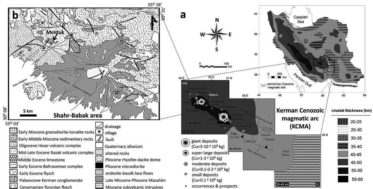
Fig. 1. Geological setting. a: Moho depths (grey shaded) and crustal thickness (km) in the KCMA with distribution and size of porphyry Cu deposits and prospects (after Saric & Mijalkovic, 1973). Inset: contour map of present-day crustal thicknesses in Iran (simplified after Dehghani & Makris, 1983; modified after Shafiei et al. , 2009); b: Geological map of the Shahr-Babak area and location of the Meiduk porphyry (modified after Dimitrijevic, 1973).
