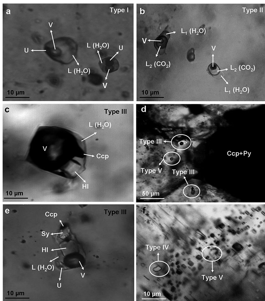
Fig. 4. Photomicrographs showing fluid-inclusion types in quartz veins of the Meiduk mine. Abbreviations: L( \text{H}_2\text{O} ) = \text{H}_2\text{O} liquid; L( \text{CO}_2 ) = \text{CO}_2 liquid; V = vapour; HI = halite; Sy = sylvite; U = unknown solid or daughter phases; Ccp = chalcopyrite; Py = pyrite. a: Type-I fluid inclusions, two-phase aqueous inclusions (liquid + vapour ± solid); b: Type-II fluid inclusions, three-phase liquid-carbonic inclusions ( \text{LH}_2\text{O} + \text{LCO}_2 + \text{V} ); c: Type-III fluid inclusions, multi-phase solid inclusions; d: Possible co-occurrence of type-III (multi-phase solid inclusions) and type-V (gaseous type) fluid inclusions in a type-B vein (boiling process) and close relationship between both types (III and V inclusions) and sulphide minerals (e.g., Ccp = chalcopyrite and Py = pyrite) in a type-B vein (stage 2); e: Type-III fluid inclusions; f: Type-IV (monophasic liquid) and type-V (monophasic gaseous) fluid inclusions in Meiduk quartz veins.
