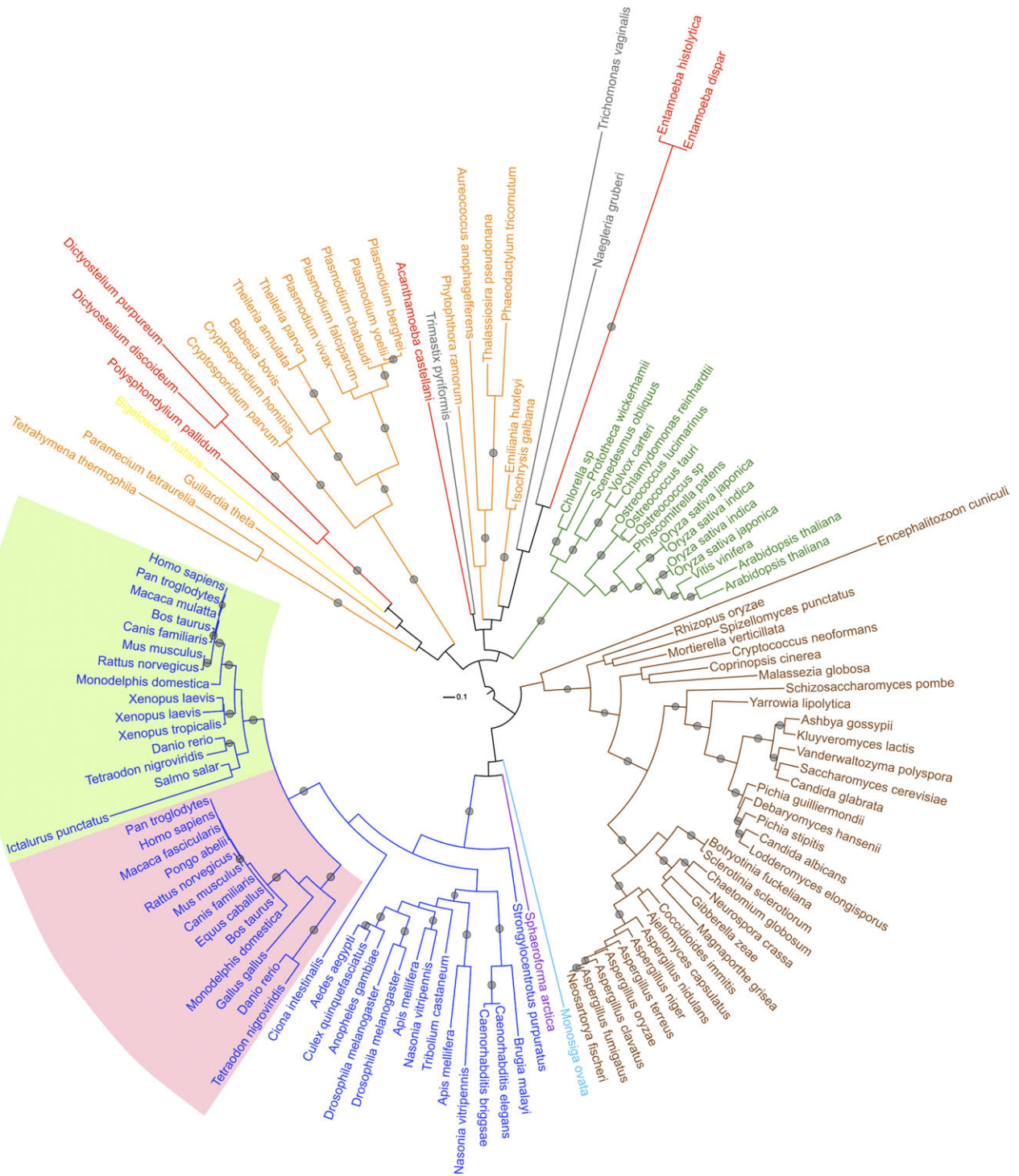
FIG. 4. —ML tree of 124 Tom40 amino acid sequences. Colors as described in figure 2. Colored leaf ranges denote two subclades created by two vertebrate Tom40 isoforms. Filled circles represent bootstrap values of 80% and above.
