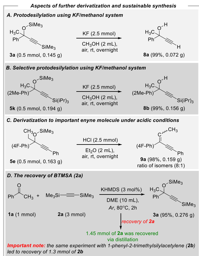
Figure 8. Potential pathways for derivatizations and rationale for the excess amount of silylacetylene.
