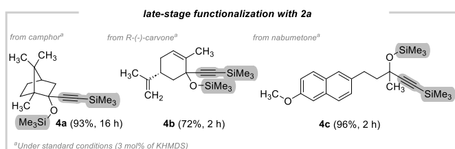
Figure 3. Late-stage functionalization of biorelevant ketones.
