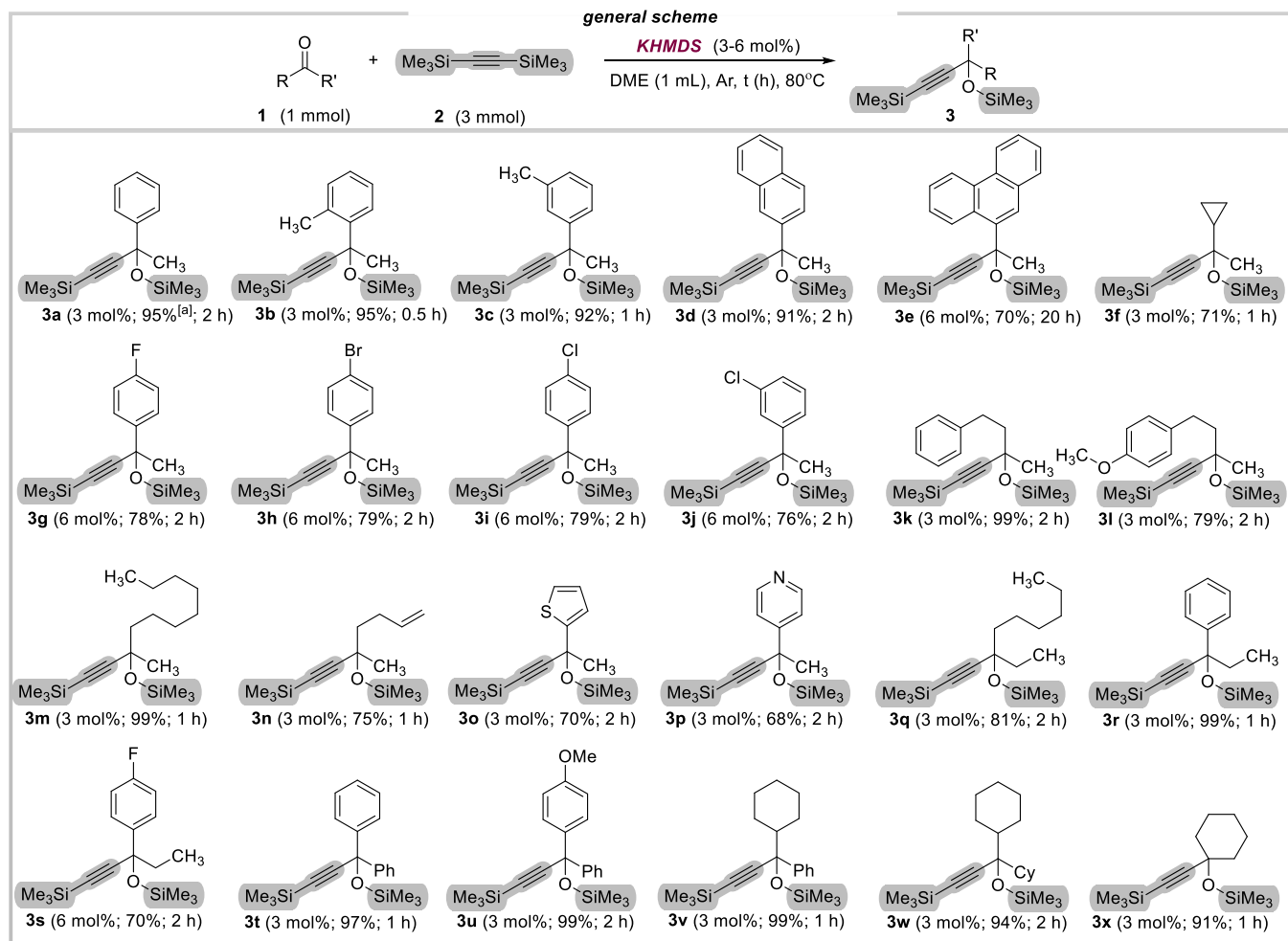
Figure 2. Substrate scope for the addition of bis(trimethylsilyl)acetylene to ketones in the presence of KHMDS.
