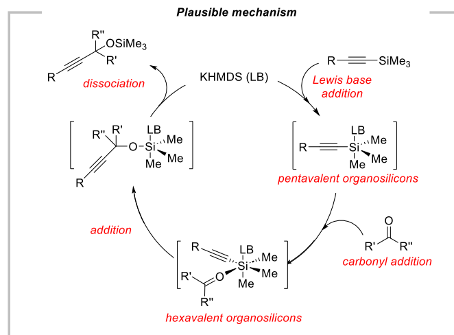
Figure 10. Plausible mechanism for KHMDS-catalyzed addition of silylacetylenes to carbonyls.
