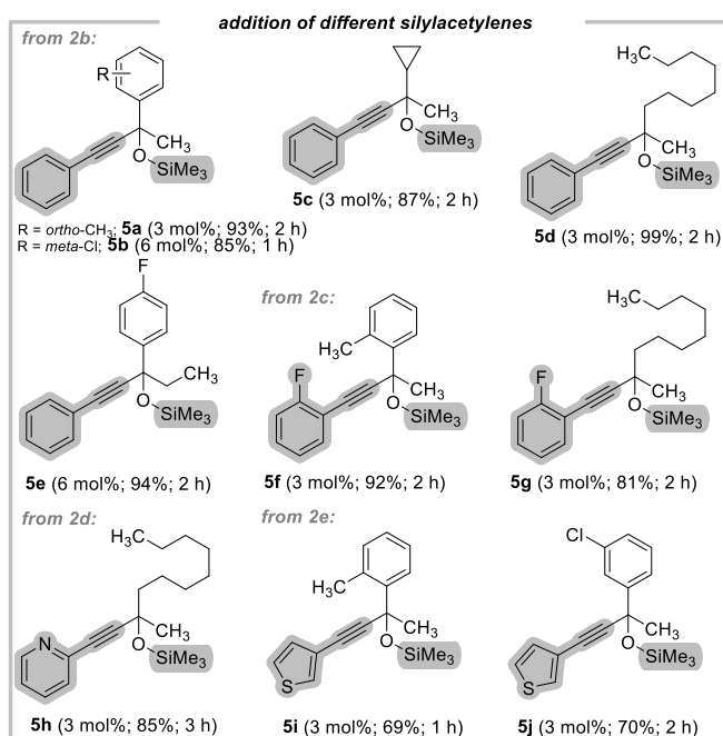
Figure 4. Substrate scope for the addition of different silylacetylenes to ketones in the presence of KHMDS.
