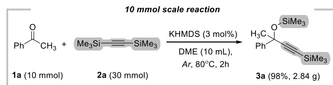
Figure 6. Scaled up synthesis of 3a .
