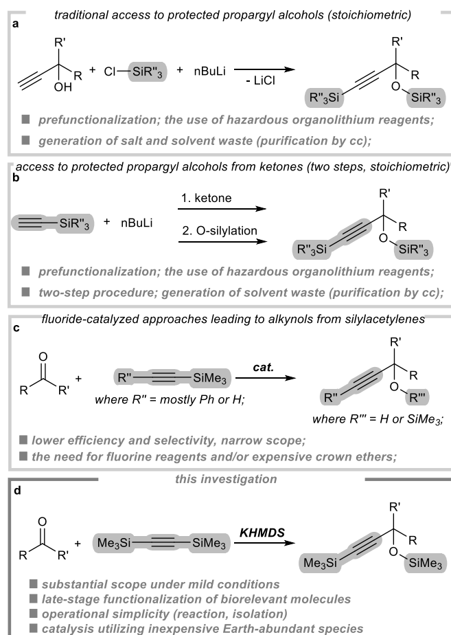
Figure 1. Context of the investigation.
