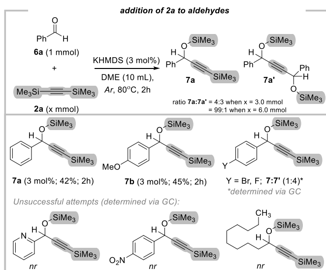
Figure 5. Initial reaction between aldehydes and BTMSA under standard conditions.
