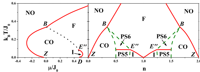
FIG. 5. Finite temperature phase diagrams for W/J = 1.5 and U \rightarrow +\infty . Denotations as in Fig. 2.
