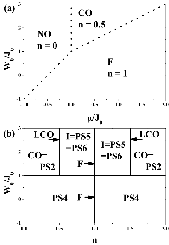
FIG. 1. Ground state phase diagrams in the U \rightarrow +\infty limit: (a) as a function of \bar{\mu}/J_0 and (b) as a function of n . Dotted lines denote discontinuous transitions (on the panel (a)).
