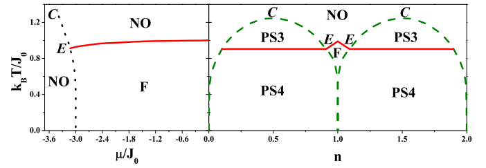
FIG. 2. Finite temperature phase diagrams for W/J = -5 (the U \rightarrow +\infty limit). Dotted, solid and dashed lines indicate first order, second order and “third order” boundaries, respectively. Details in text.
