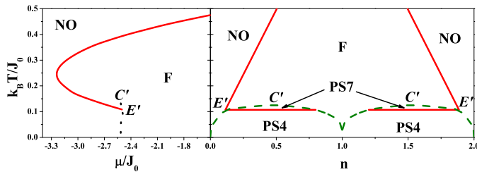
FIG. 4. Finite temperature phase diagrams for W/J = 0.5 and U \rightarrow +\infty . Denotations as in Fig. 2.
