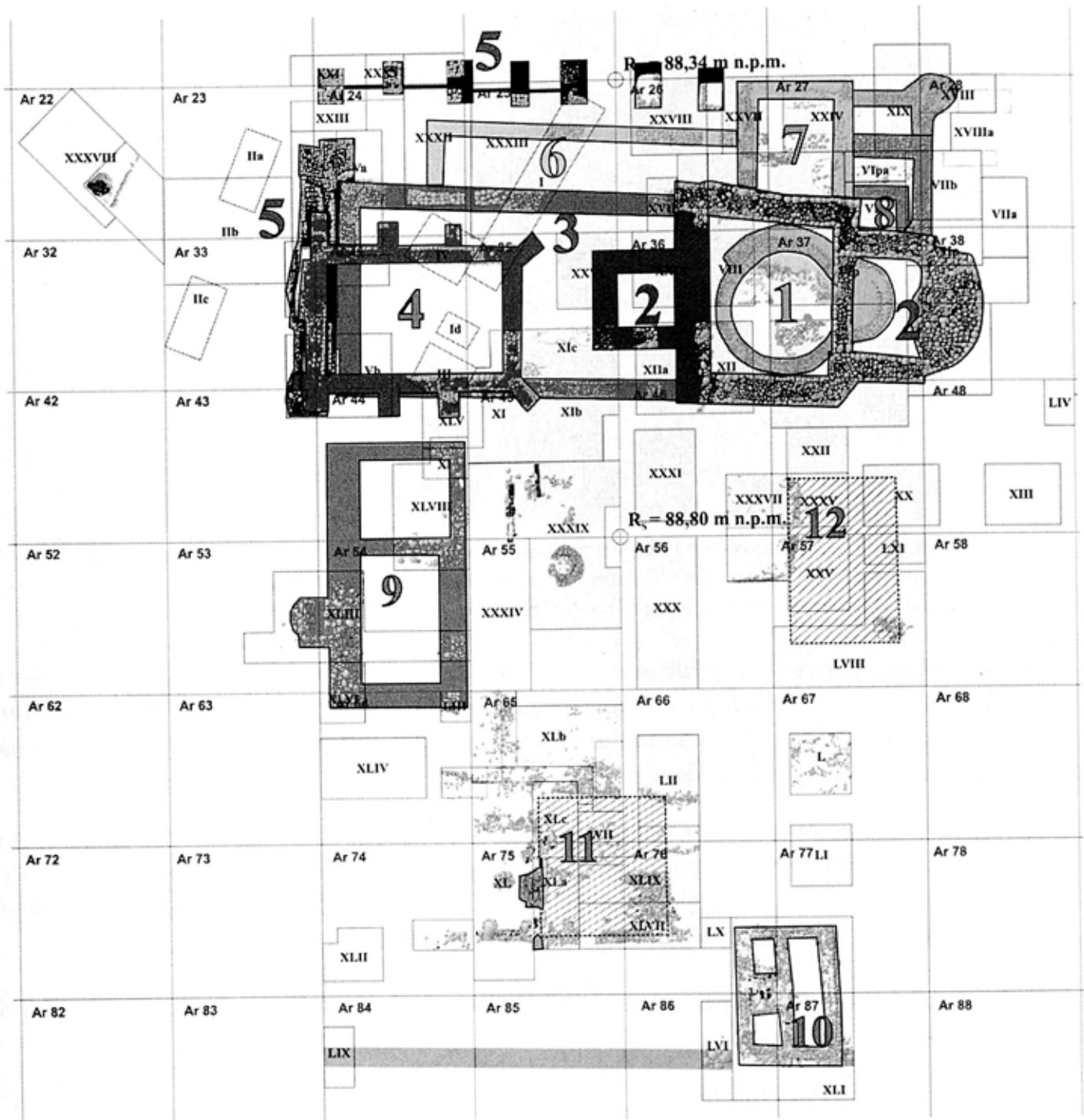
Figure 3 Plan of basement of architectural objects in Łekno site Ł3. The remnants of settlement walls have not been taken into account (the settlement is situated below the objects 1–9, 12, and partly 11): 1 – rotunda; 2 – Cistercian church, phase A1 (oratory); 3 – Cistercian church, phase A2 (full-scale church, connected with phase A1); 4 – cemetery chapel, middle 15th cent.; 5 – Phase A2-2 of Cistercian church; 6 – chapels of phase A2; 7 – vestry, phase A2; 8 – vestry, phase A1; 9 – dormitorium; 10 – so-called “abbot’s house”; 11 – kitchen and refectory; 12 – remnants of chapter house.
